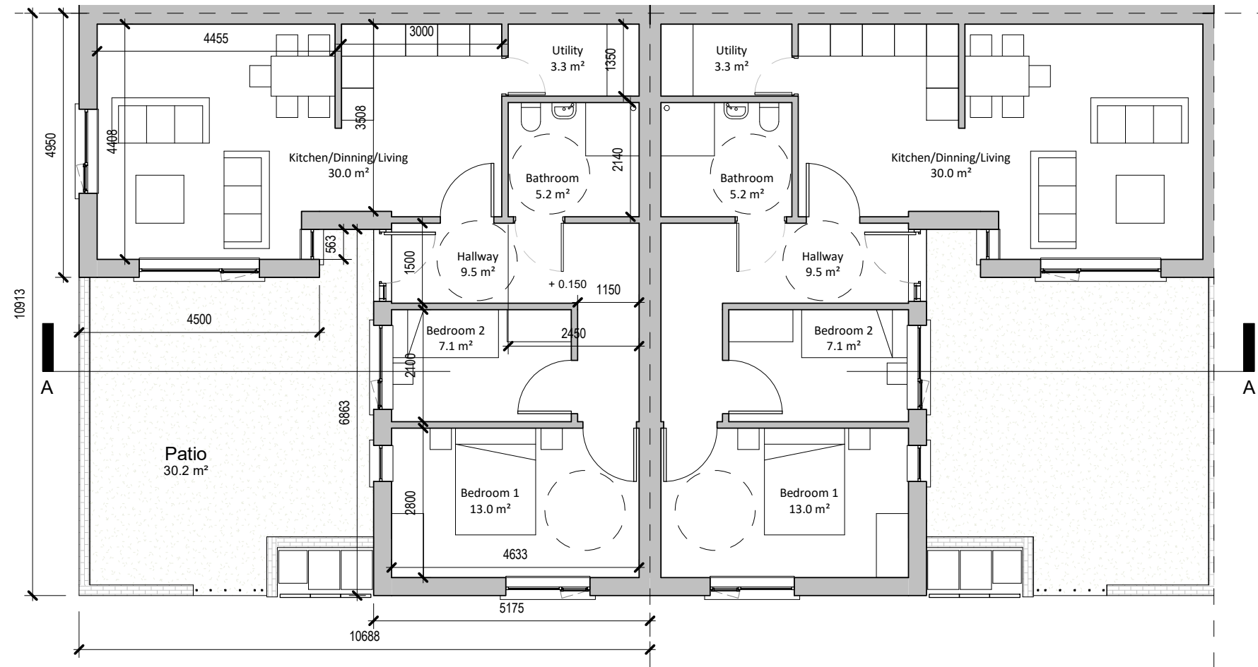
① H09A - Ground Floor - End & Mid Terrace 1 : 100
